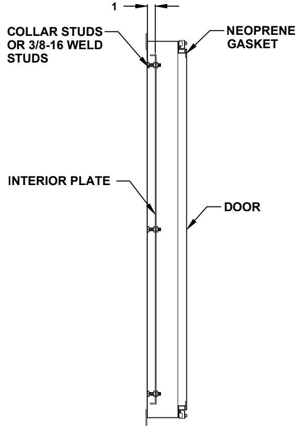
CROSS SECTION VIEW A-A
