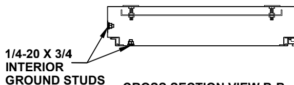
CROSS SECTION VIEW B-B
