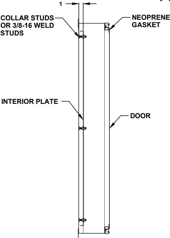
CROSS SECTION VIEW A-A
