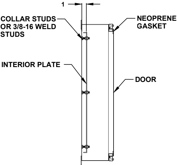
CROSS SECTION VIEW A-A
