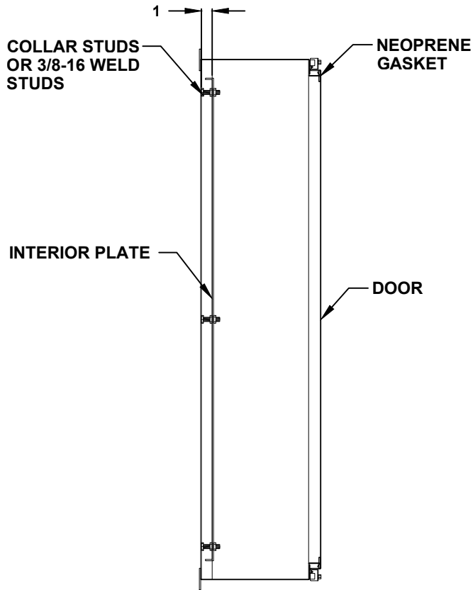
CROSS SECTION VIEW A-A
