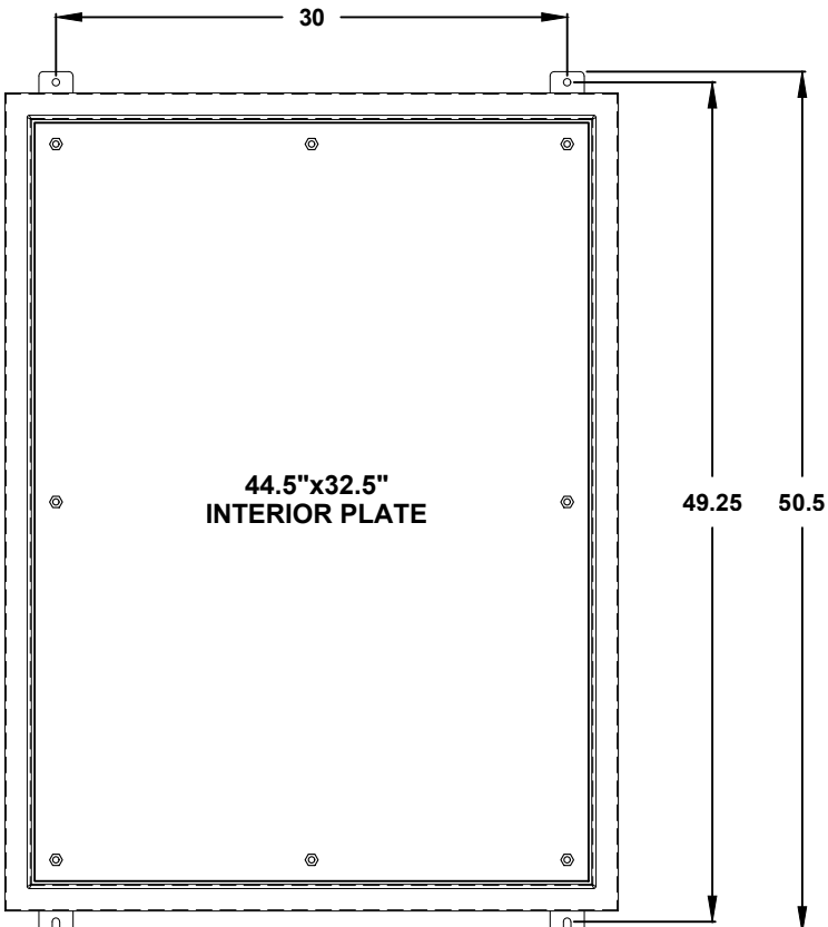
FRONT VIEW WITH DOOR REMOVED
