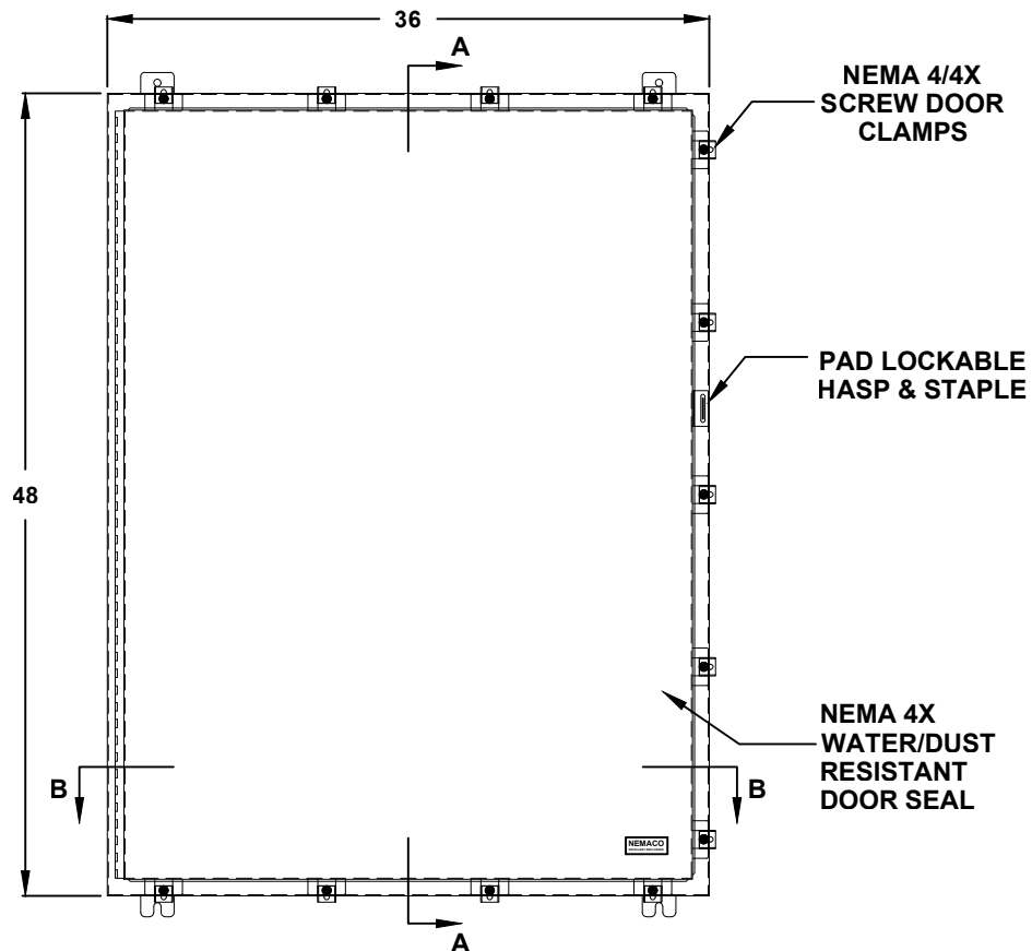
FRONT VIEW
