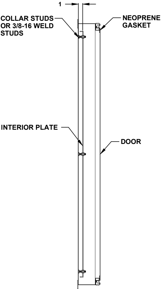
CROSS SECTION VIEW A-A
