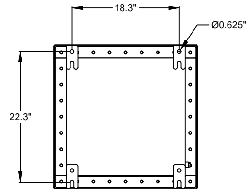
BACK VIEW
