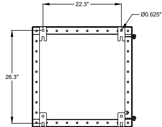
BACK VIEW
